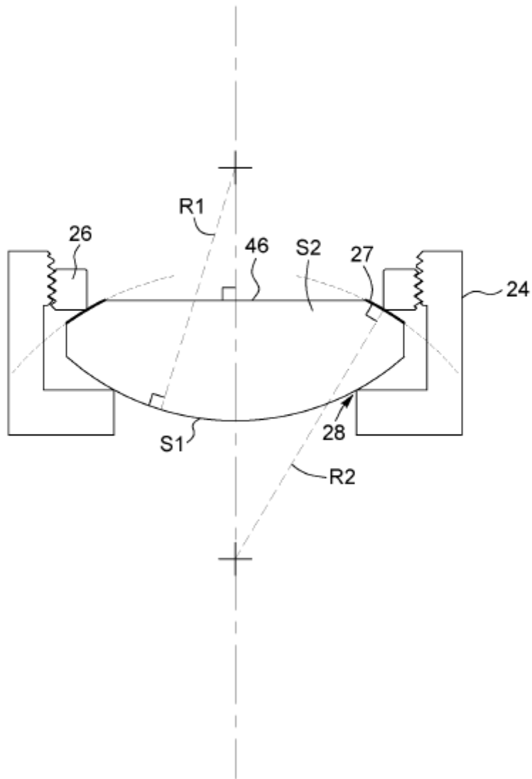
FIG. 11D
