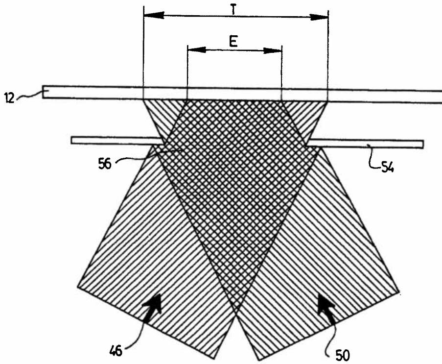
FIG. 6A LARGE SLIT
