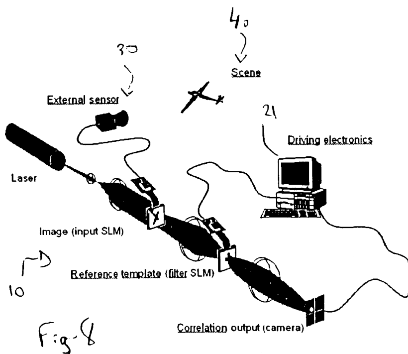
Optical correlator system illustration.
