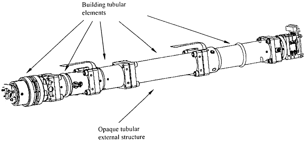
Figure 2: Perspective view of the tubular optical correlator
