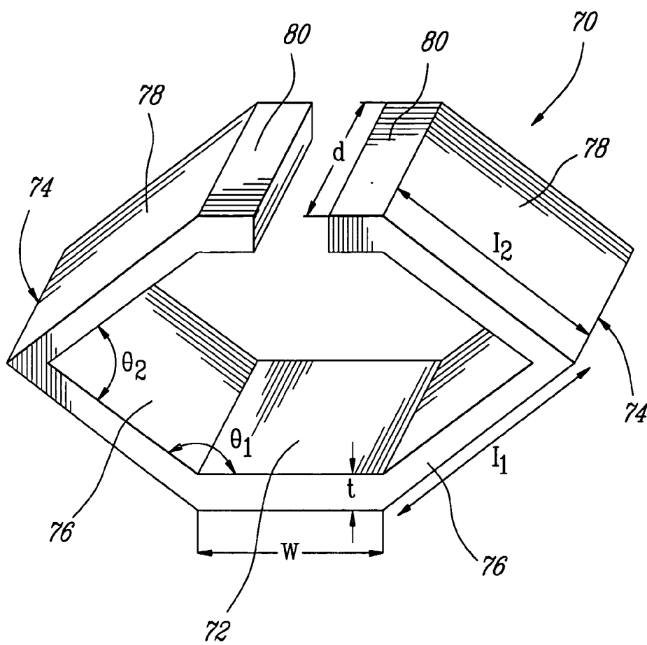
Fig. 7 (PRIOR ART)
