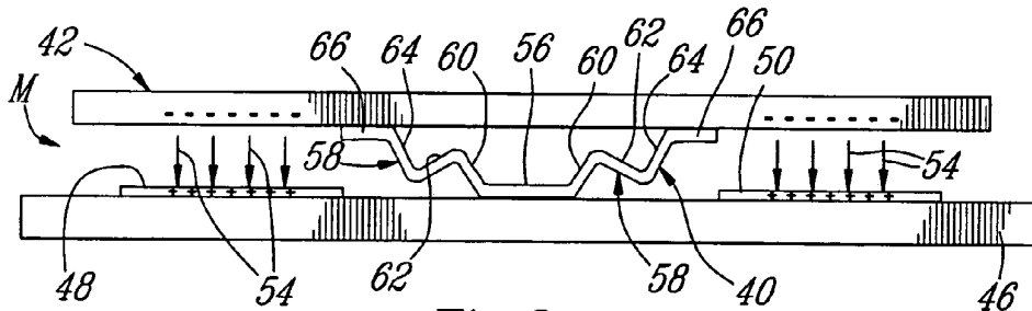
Fig. 3c (PRIOR ART)
