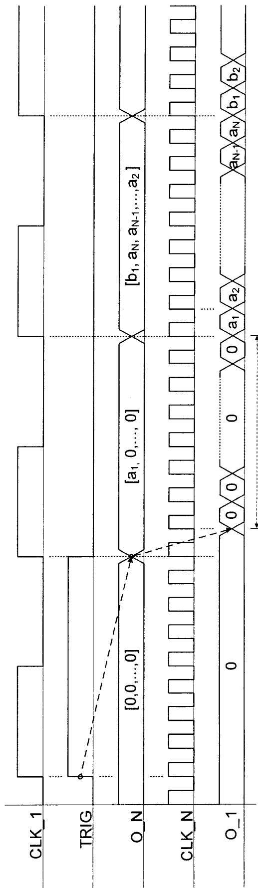
\text{FINE\_DELAY} = (N-1) FIG. 6D
